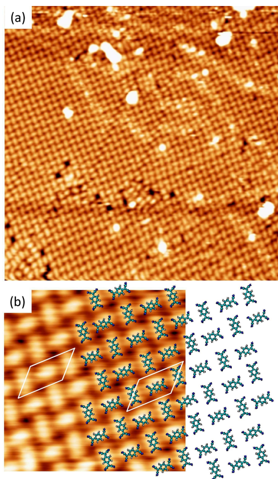
Fig. 3 (a) STM overview ( 400 \text{ \AA} \times 400 \text{ \AA} ) acquired with V_s = -1 \text{ V} and I_t = 0.08 \text{ nA} displaying highly ordered compact structure of TCNQ/Cu(111), performed by deposition on Cu(111) held at 350 K. (b) High resolution STM image ( V_s = +1 \text{ V} , I_t = 0.08 \text{ nA} ) of the orthogonal compact structure. A proposed model of the structure (considering non-deformed molecules) is represented and superimposed over the STM image. The white parallelogram with a lateral size of 16 \text{ \AA} and 8 \text{ \AA} measured from the STM images represents the unit cell.
