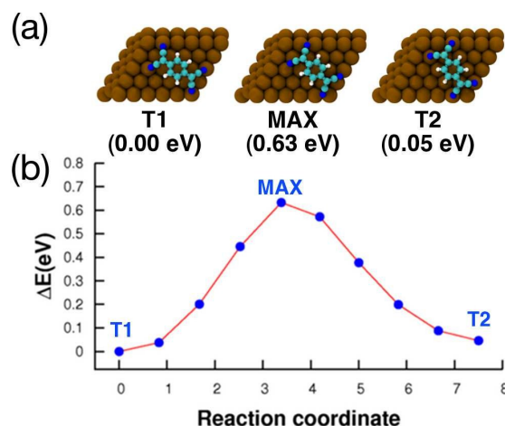
Fig. 5 (color on line) Interconversion between the two adsorption configurations shown in Figure 4, calculated using the CI-NEB method. (a) Top view of the geometries and energies relative to the most stable adsorption configuration (T1), the configuration at the maximum of the barrier (MAX), and the second most stable configuration (T2). Cu, C, N and H atoms are printed in brown, cyan, blue and white, respectively. (b) Reaction path for the interconversion. In both axis, the 0 is placed at the most stable adsorption configuration.
