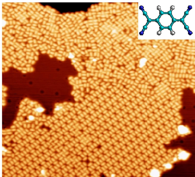
Fig. 1 STM image ( 450 \text{ \AA} \times 410 \text{ \AA} ) displaying the TCNQ arrangement after deposition at room temperature. V_s=+1 \text{ V} and I_t=0.1 \text{ nA} . Inset: Schematic ball-and-stick representation of TCNQ molecule.
