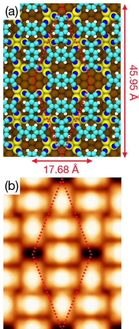
Fig. 7 (a) Optimized geometry of the complex structure obtained at the DFT+D2/PBE level of theory. Colour code for atoms is the same as in figure 4. (b) Simulated STM topography of the same structure for an applied bias voltage V_s = +1.0 V.
