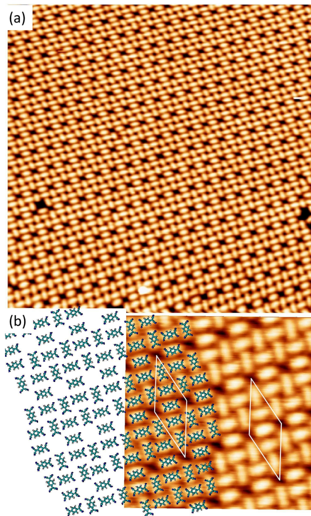
Fig. 2 (a) STM image ( 500 \text{ \AA} \times 500 \text{ \AA} ) acquired with V_s=+1.4 \text{ V} and I_t=0.3 \text{ nA} displaying highly ordered structure of TCNQ/Cu(111). The TCNQ molecules are deposited with the substrate at room temperature and afterwards a short annealing at 350K is done. (b) High resolution STM image of the complex structure ( V_s=+1 \text{ V} and I_t=0.1 \text{ nA} ). A proposed model of the structure (considering non-deformed molecules) is represented and superimposed over the STM image. The white rhomb with a long diagonal of 47.6 \text{ \AA} and the short one of 19.5 \text{ \AA} represents the unit cell.
