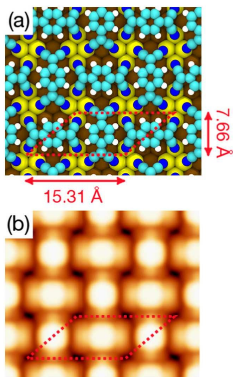
Fig. 8 (color on line) (a) Optimized geometry of the orthogonal structure monolayer obtained at the DFT+D2/PBE level of theory. Color code for atoms is the same as in figure 4. (b) Simulated STM topography of the same structure for an applied bias voltage V_s = +1.0 V.
